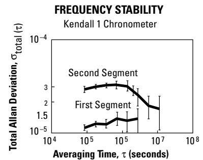
Figure B6. A plot of the frequency stability for the data taken in each of the two galleries. K-1 was about a factor of two less stable during its time in the second gallery than in the first. Notice the hump in the stability plot for \tau values of the order of one to two weeks. This is apparently due to the steps in frequency occurring every few weeks. Notice also that the long-term \tau = 128 days value is almost in line with extrapolated stability curve from the first segment. In other words, it appears that whatever caused K-1’s rate to go high for a few days, this effect tended to average out over long enough time—a very good attribute.
