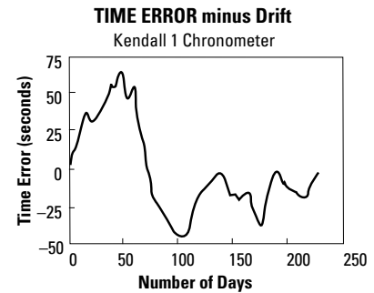
Figure B5. After subtracting a frequency drift as estimated from K-1’s frequency data by simple linear regression, the residual time errors were calculated and are plotted here. In this case, as compared to Figure B4, the time errors are only reduced by a little over a factor of two. How much the timing errors will be reduced by frequency drift calibration is a function of the size of the drift as compared to the random clock noise. Calibrating frequency drift in quartz-crystal oscillators and rubidium gas-cell frequency standards is often very beneficial. It is not surprising that there is some frequency drift in a mechanical timing device.
